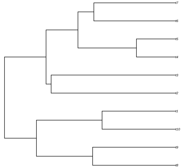
true_tree
